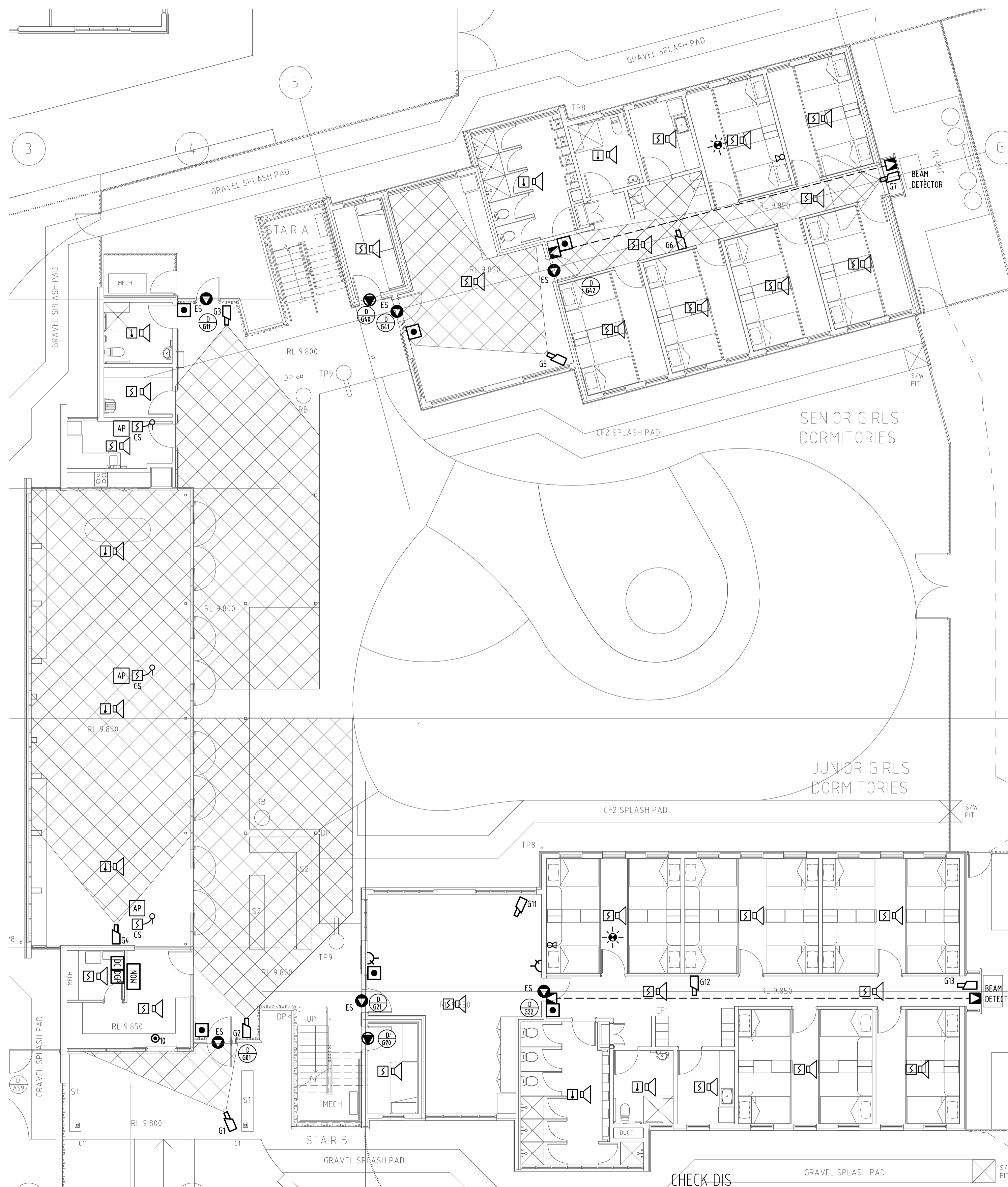
GROUND FLOOR
