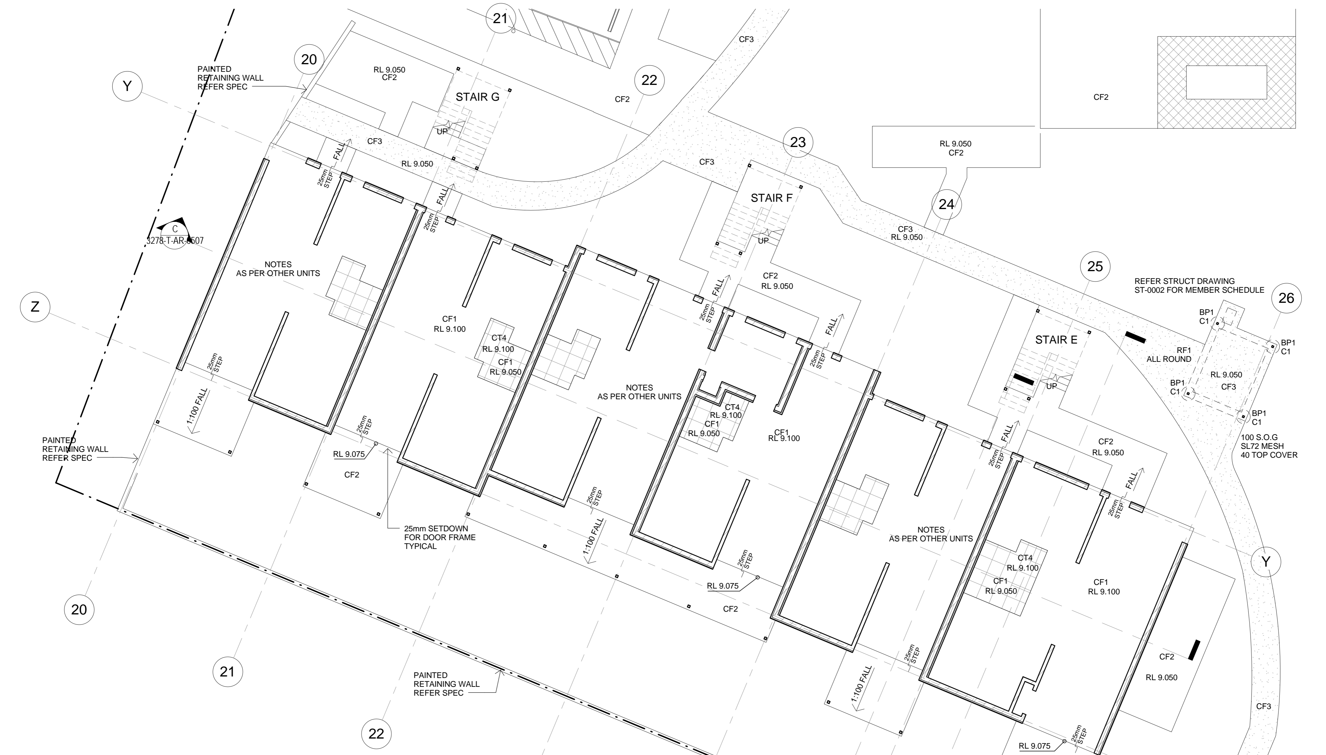
STAFF ACCOMODATION - GROUND FLOOR STRUCTURAL SETOUT
